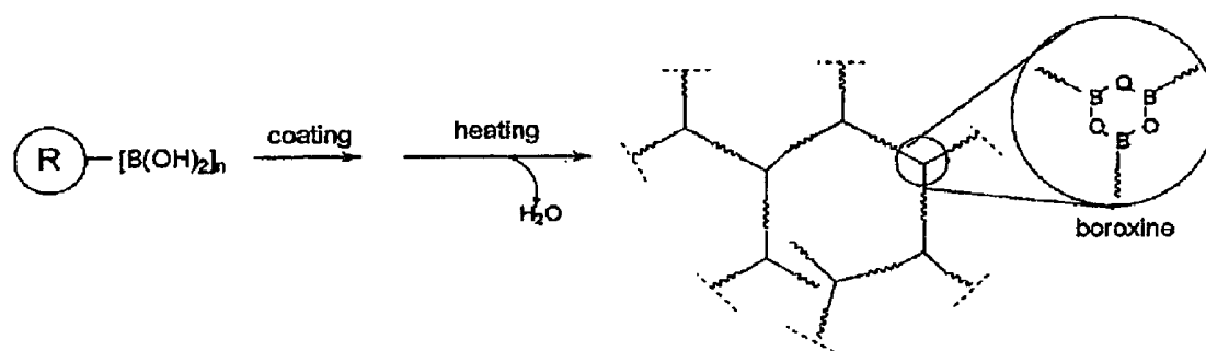
Crosslinked networks
