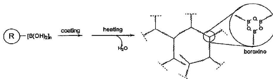
Crosslinked networks
