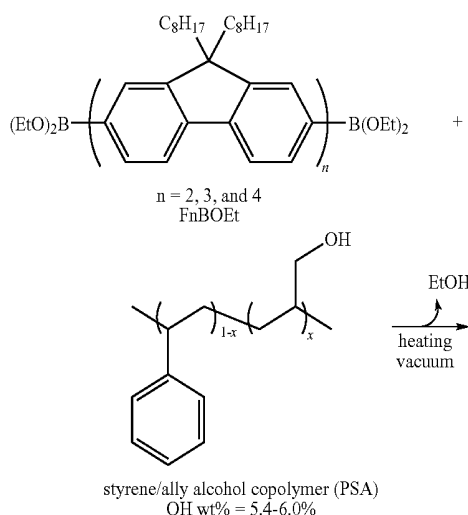
Scheme 3. Formation of blue-light emitting networks via transesterification of FnBOEt with PSA.
