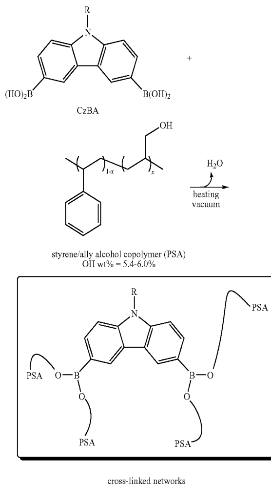
Scheme 1. Formation of hole-transporting networks via esterification of CzBA with PSA.
