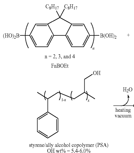
Scheme 2. Formation of blue-light emitting networks via esterification of FnBA with PSA.
