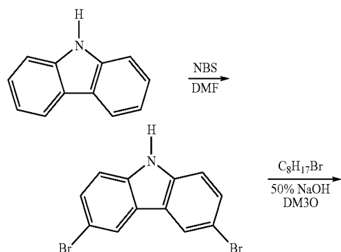
Scheme 3. Synthesis of hole-transporting boronic acids
